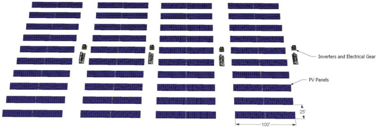
Figure 5. - Proposed Ground-Mounted PV Installation for One Megawatt Capacity
