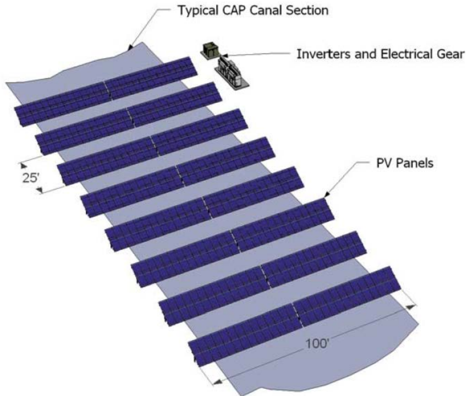
Figure 4. - Proposed CAP Canal PV Installation for One Megawatt Capacity (only a portion of the modules shown)
